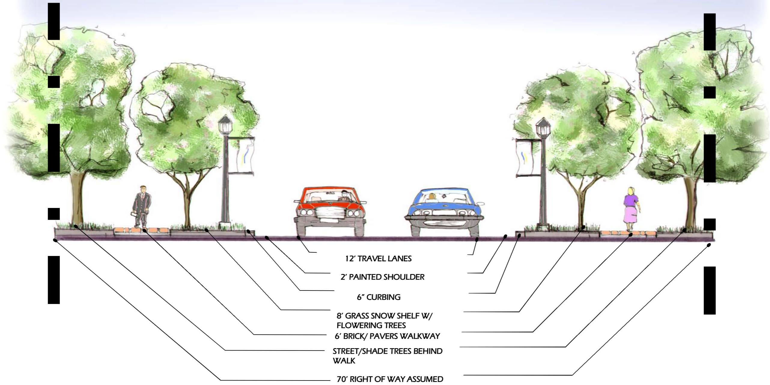
TYPICAL TRAFFIC CALMING ROAD SECTION
